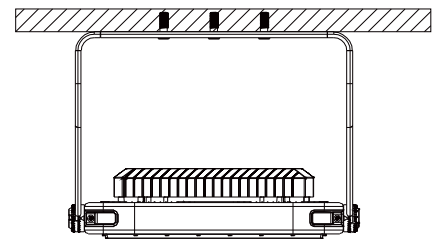
Hanging Mounting
